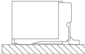
Assembly Layout
